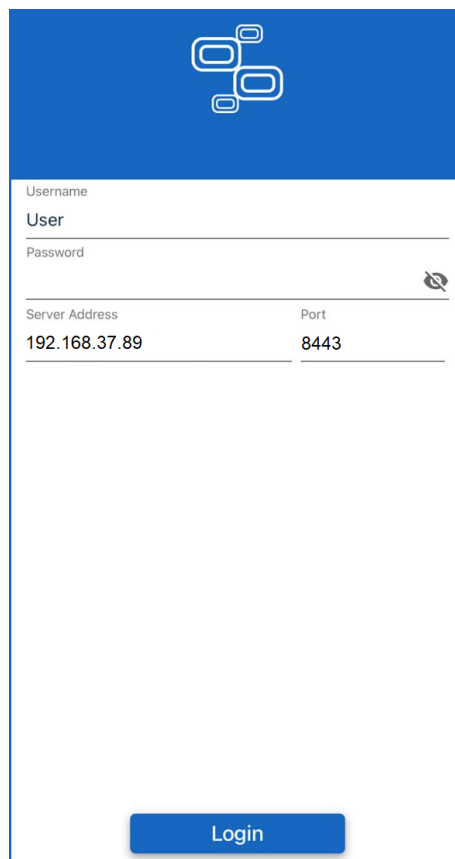
Fig. 2. SmartPTT Mobile Login Screen
